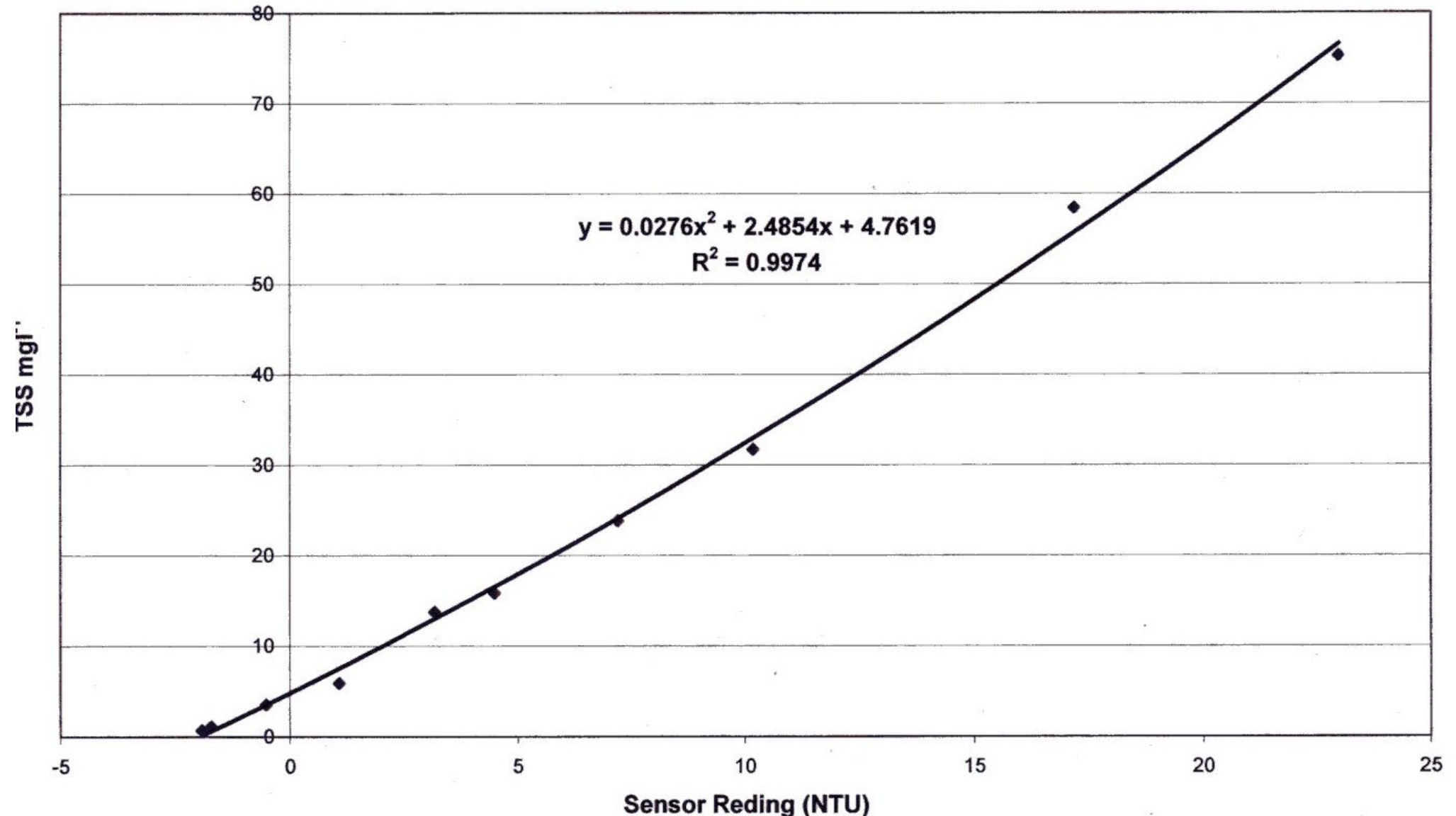
TSS Calibration Graph
